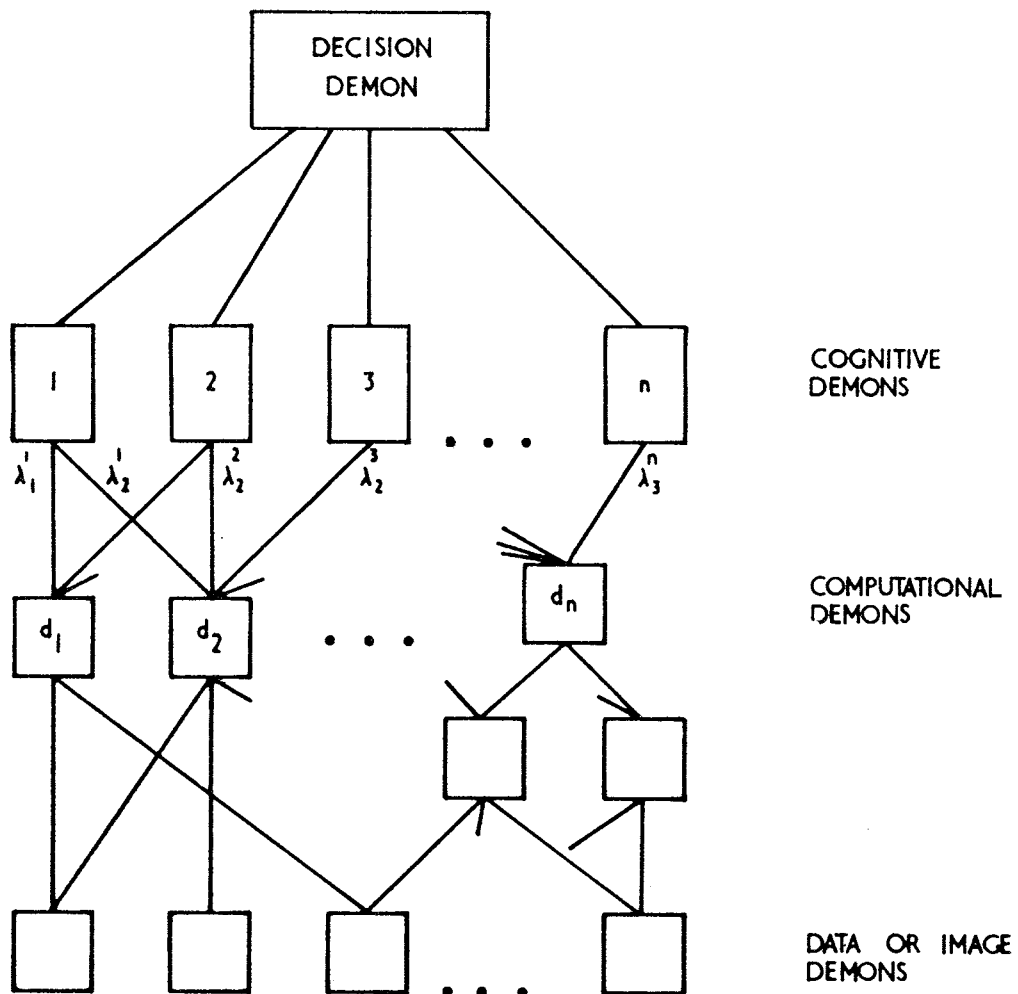
Fig. 3. Amended Pandemonium
