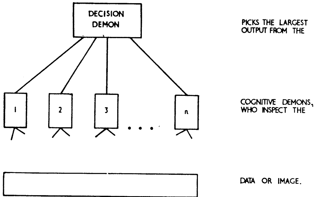
Fig.1. Idealized Pandemonium.
